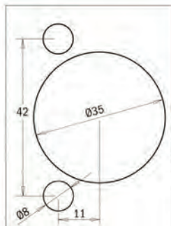
1 CMT333-4211 per cerniera Grass 42/11 para bisagra Grass 42/11
